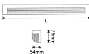
CAB 3/CAB 3N
