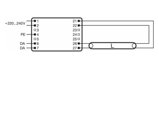
Wiring diagram
