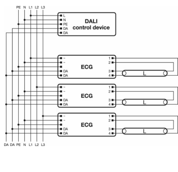
Wiring diagram
