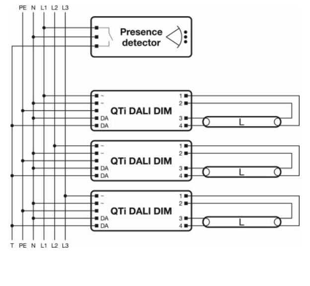
Wiring diagram
