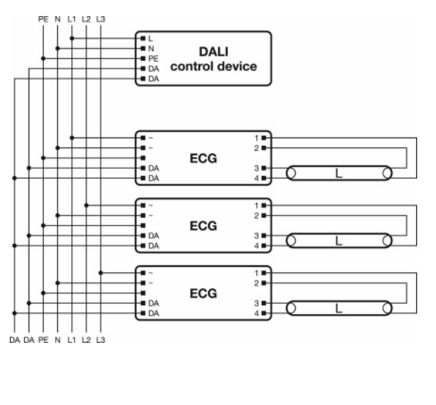
Wiring diagram
