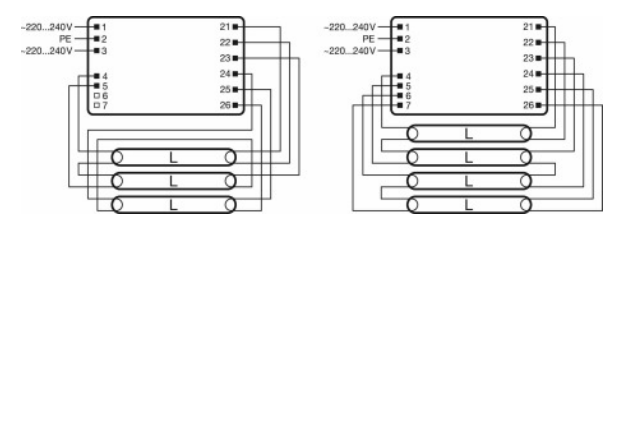
Wiring diagram
