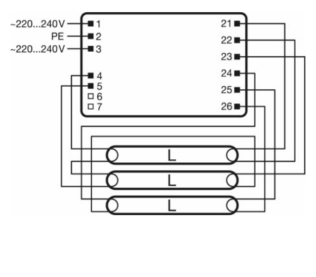
Wiring diagram
