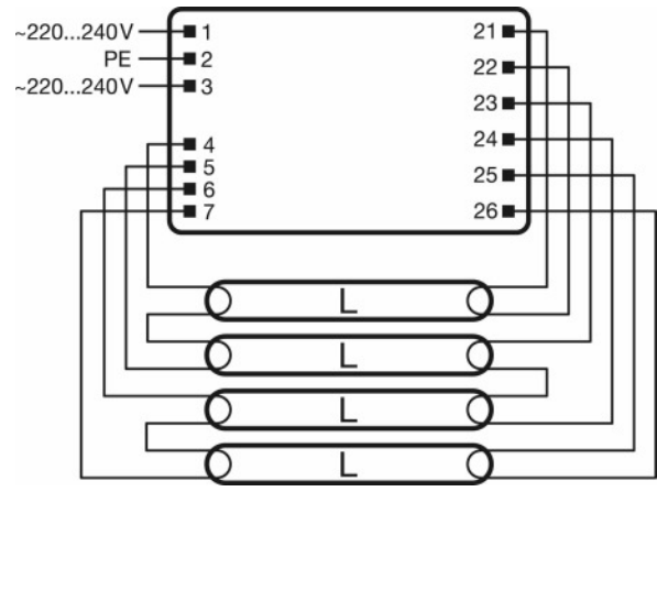
Wiring diagram
