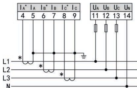
3P 4W, 3CT, без PT
