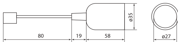
SQ0335-0021, SQ0335-0023
