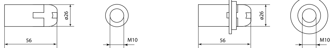
SQ0335-0009, SQ0335-0032, SQ0335-0053, SQ0335-0057
