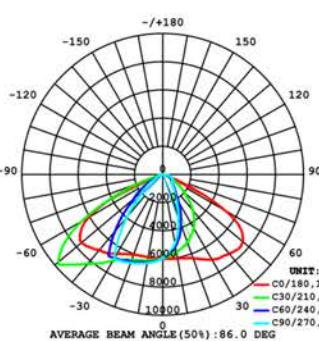
FL-LED Street 200W
