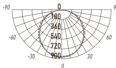
PWP-C2 1200 40w
