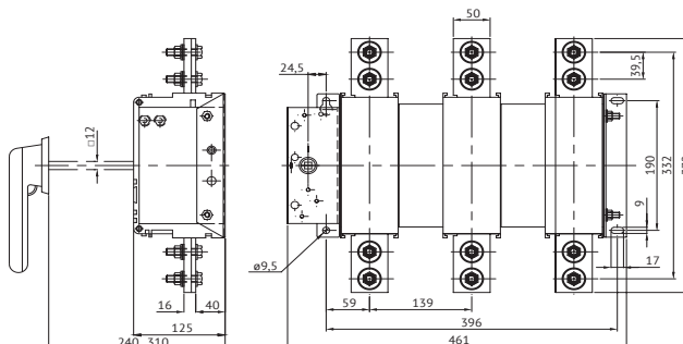
OptiSwitch DI-5-(1600-1800A)
