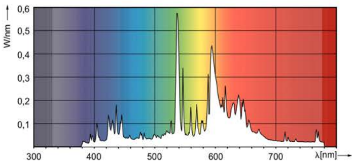
LDPO_CDO-TT_0002-Spectral power distribution Colour
