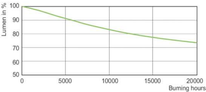
MASTER CityWhite CDO-ET Plus CDO-TT Plus 70W/828 E27
