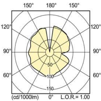
LDLD_CDO-TT_0001-Light distribution diagram
