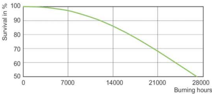
LDLE_CDO-TT_0001-Life expectancy diagram
