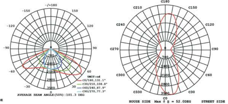
FL-LED Street-Garden 100W
