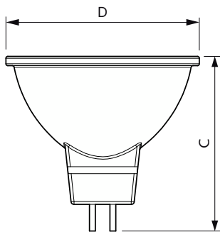
ESS LEDspot 5W 400lm GU5.3 865 220V
