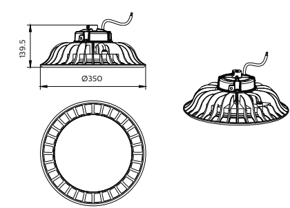
SmartBright High-bay BY218P/BY235P
