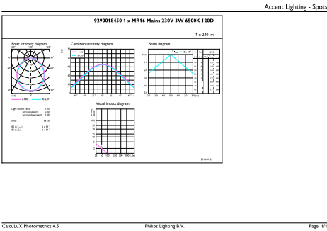
LEDspot ESS 35W GU5.3 MR16 865 12D ND RCA
