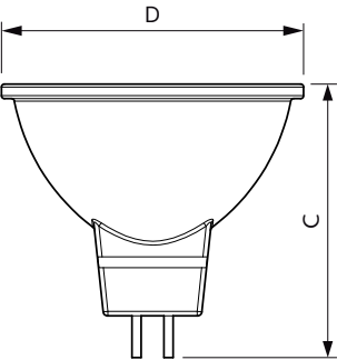
MR16 12V 3W-35W 230lm 120D 6500K GU5.3
