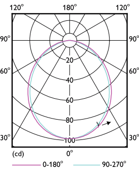
LEDspot ESS 35W GU5.3 MR16 827 12D ND RCA
