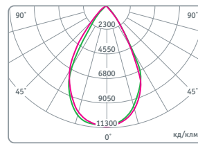
NHB-P7-100-5K-60D
