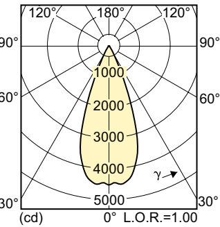
LDLD_CDMR111E_0003-Light distribution diagram
