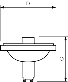
CDM-R111 Elite 35W/930 40D
