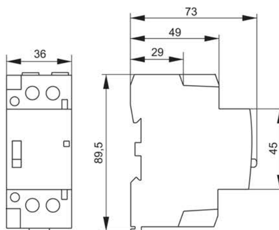
Контакторы KM63-20MP AC, KM63-11MP AC, KM40-20MP AC и KM40-11MP AC
