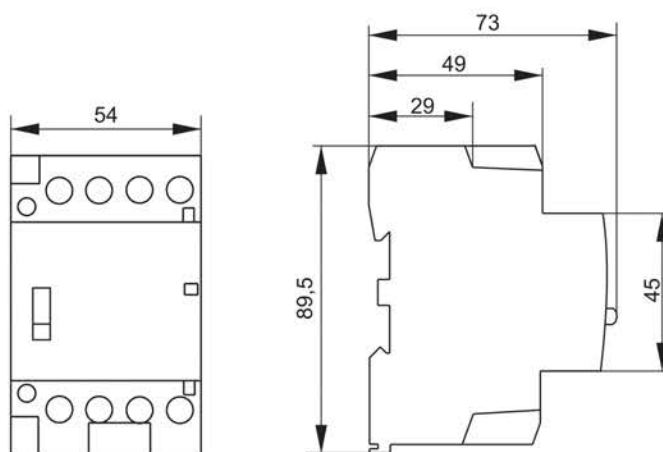
Контакторы KM25-40MP AC, KM40-40MP AC и KM63-40MP AC
