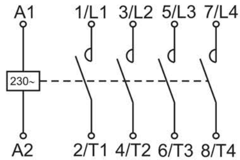
KM20-40M AC
