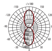
PWL-26090/24D 2x5w
