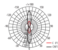
PWL-245110/24D 2x12w
