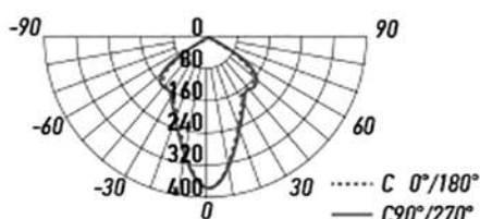
PSP-S 211 1x8W
