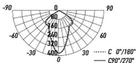
PSP-S 211 1x8W
