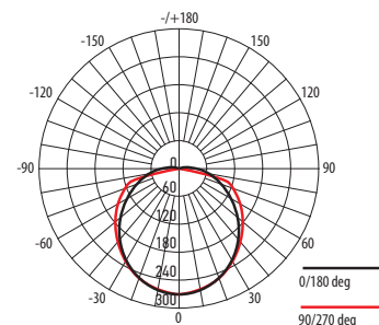
PBH-PC2-RS 12W IP65 Sensor
