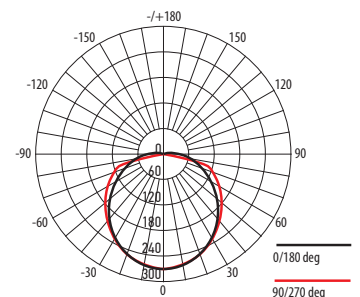
PBH-PC2-RS 12W IP65 Sensor
