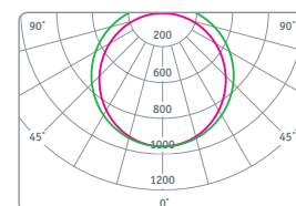
DSP-02-36-4K-IP65-LED
