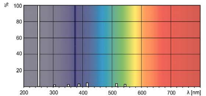
XDPB_XUTUVTLD-Spectral power distribution Colour
