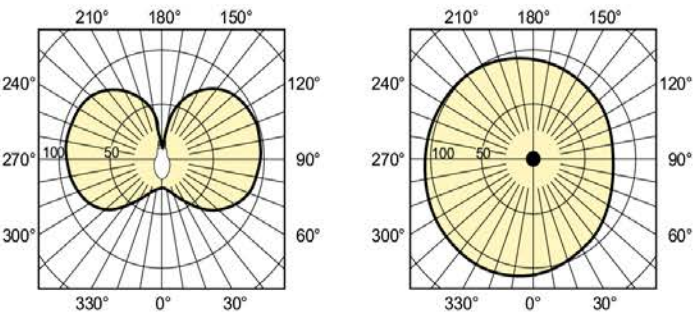
LDLD_HPI-Light distribution diagram
