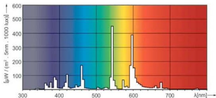
LDPO_HPI_Plus_250W_400W-Spectral power distribution Colour
