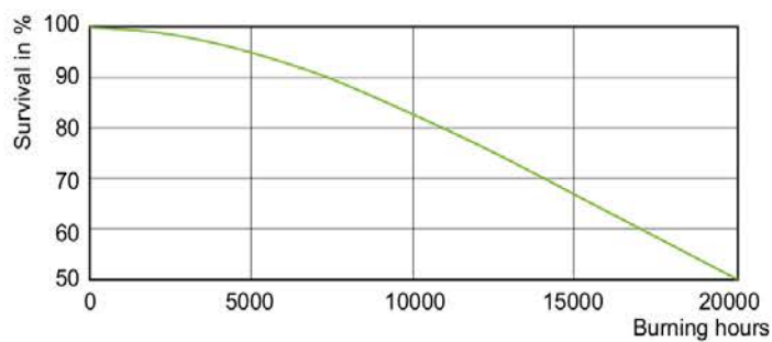
LDLE_HPI_250W_400W-Life expectancy diagram
