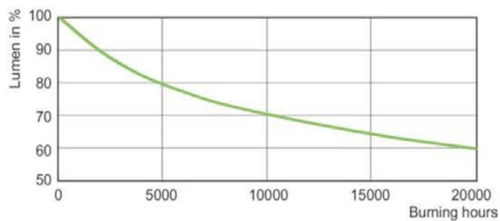
LDLM_HPI_250W_400W-Lumen maintenance diagram
