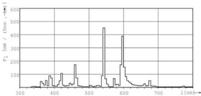
LDPB_HPI_Plus_250W_400W-Spectral power distribution B/W
