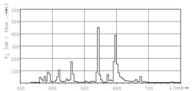
LDPB_HPI_Plus_250W_400W-Spectral power distribution B/W
