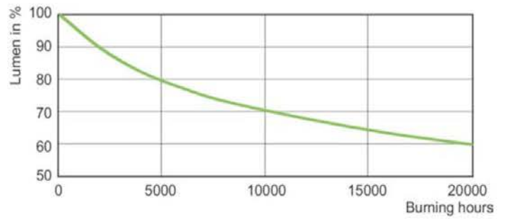
LDLM_HPI_250W_400W-Lumen maintenance diagram
