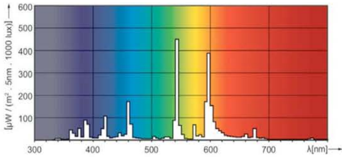
LDPO_HPI_Plus_250W_400W-Spectral power distribution Colour
