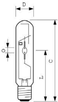
CDO-TT Plus 100W/828 E40
