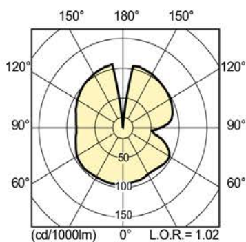
LDLD_CDO-TT_0002-Light distribution diagram
