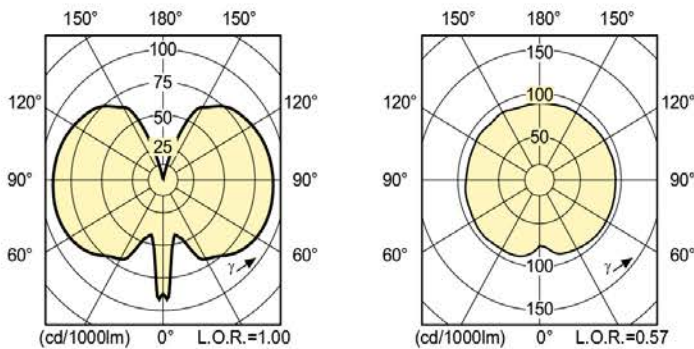
LDLD_CDM-T-E_0006-Light distribution diagram
