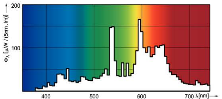
LDPO_CDM-T-E_100W_930-Spectral power distribution Colour
