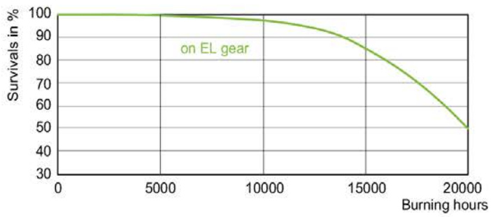
LDLE_CDM-T-E_0006-Life expectancy diagram
