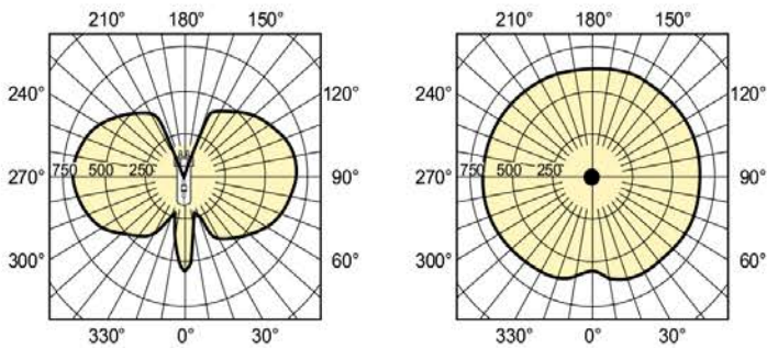
LDLD_CDM-T_70W_830_942-Light distribution diagram
