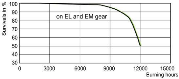
LDLE_CDM-T_70W_830-Life expectancy diagram
