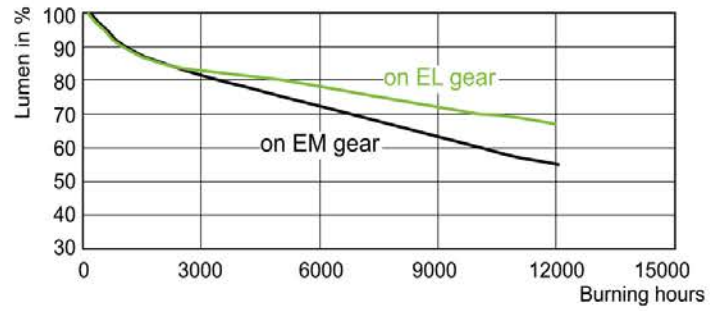
LDLM_CDM-T_70W_830-Lumen maintenance diagram
