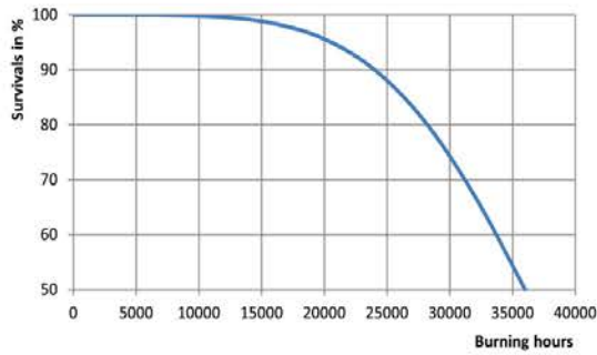
SON(-T) PIA Plus 150W 250W 400W Life Expectancy Diagram
