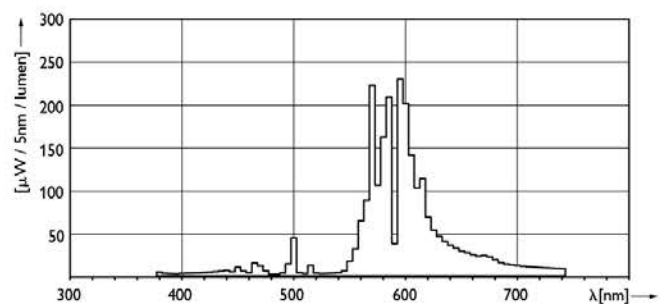
LDPB_SON-TPIA_0012-Spectral power distribution B/W
