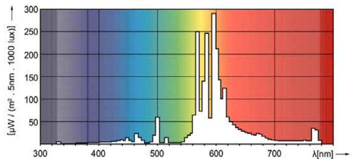
LDPO_SON-T-Spectral power distribution Colour
