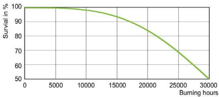
LDLE_SON-T_0001-Life expectancy diagram
