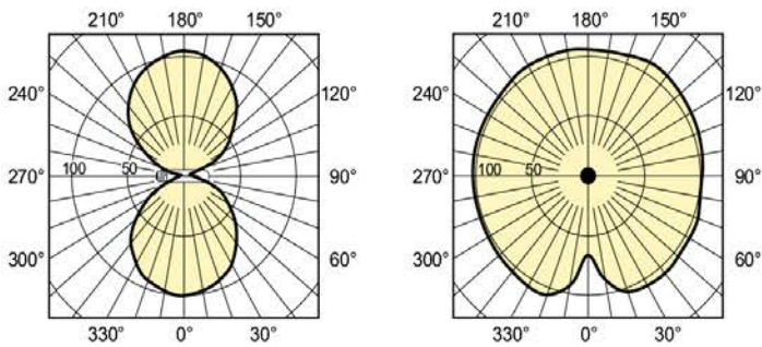
LDLD_SON-T-Light distribution diagram
