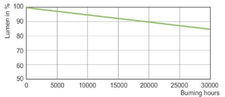
LDLM_SON-T_0001-Lumen maintenance diagram
