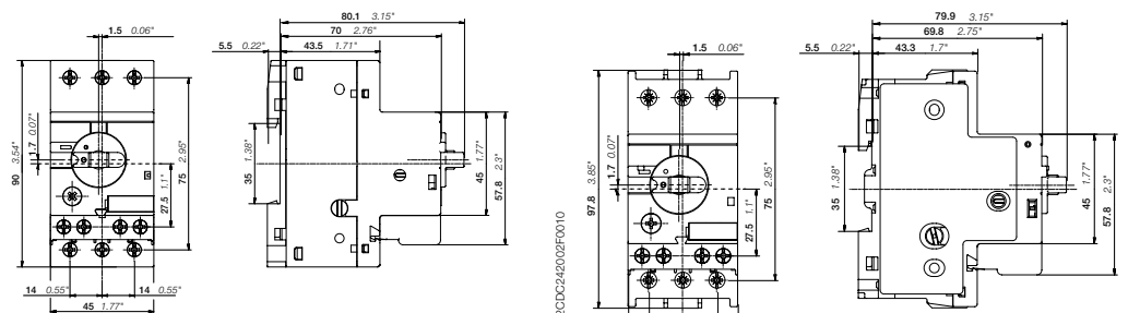
MS116 ≤ 16 A
