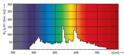
MASTERColour CDM-T 35W /842
